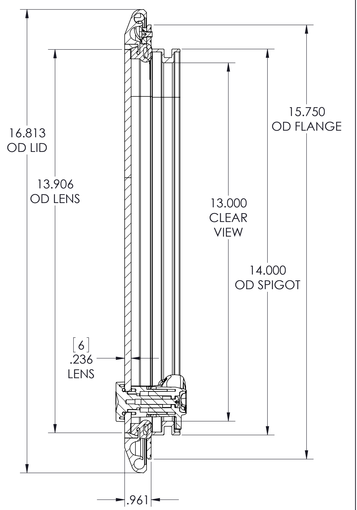
SECTION B-B
